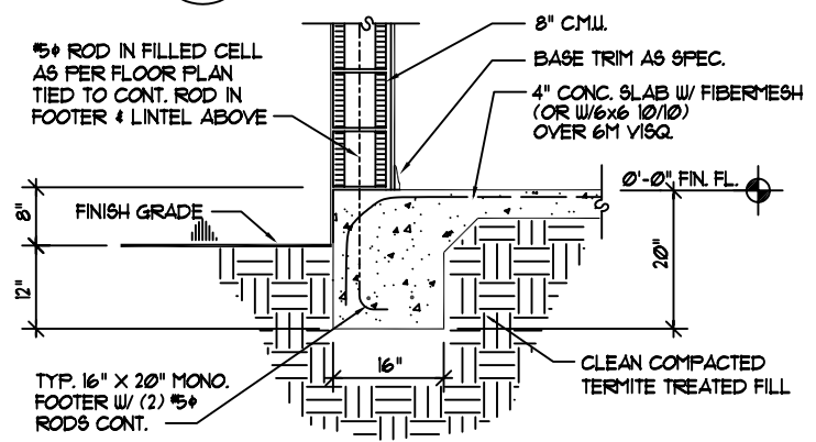
OPTIONAL MONOLITHIC FOOTING DETAIL SCALE: 3/4"=1'-0" 14A
