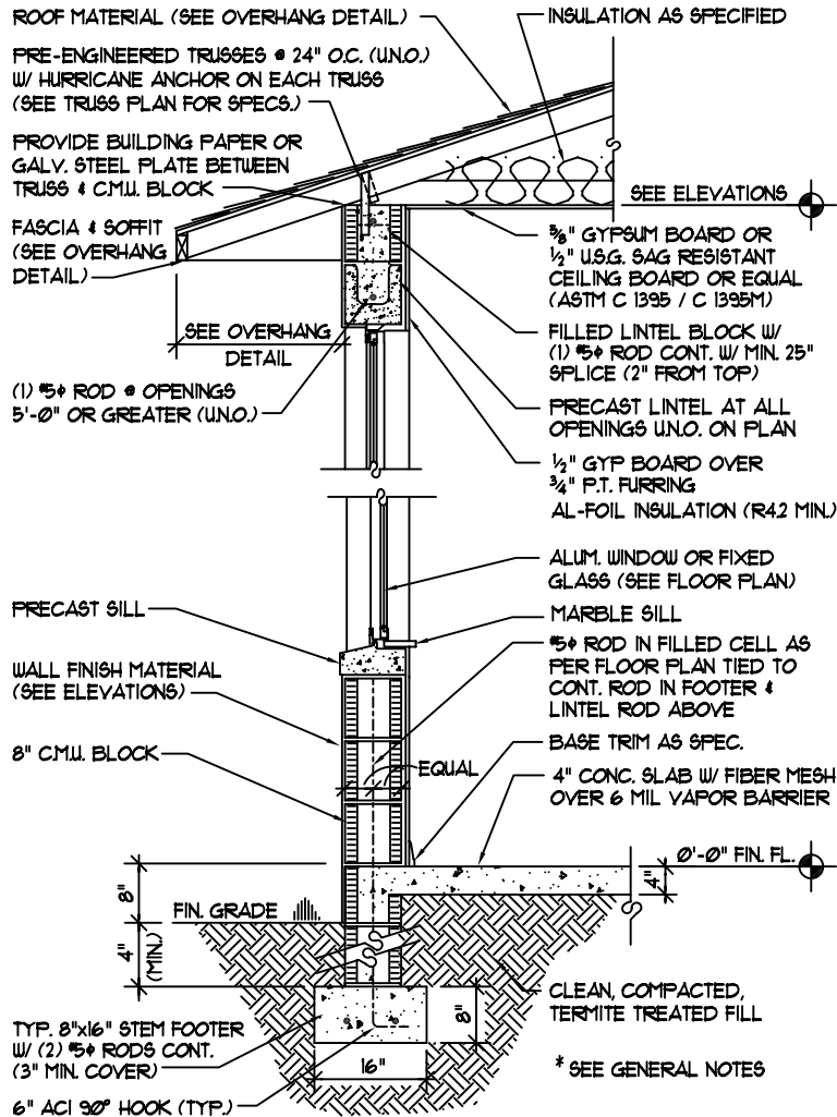
TYPICAL ONE-STORY 8" CMU BLOCK WALL SECTION SCALE: 3/4"=1'-0" 12B
