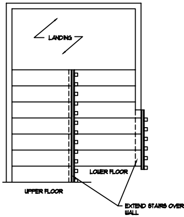
U-STAIR (PLAN) SCALE- 1/2"=1'-0" (1)
