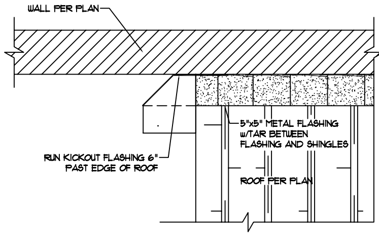
TYPICAL ROOF TO WALL FLASHING DETAIL N.T.S. PLAN VIEW
