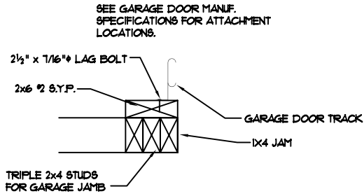
GARAGE DOOR FRAME ATTACHMENT DETAIL SCALE: 2"=1'-0"
