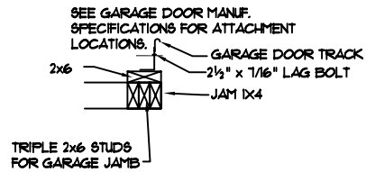
GARAGE DOOR ATTACH SCALE: 3/4"=1'-0"
